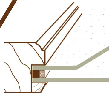
3 - 6 - 4 Glazing configuration. Textured and safety glass available
